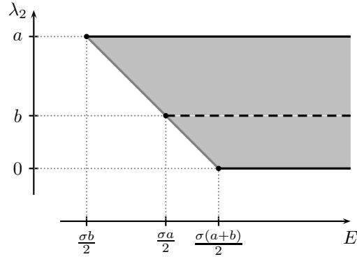
FIGURE 1. Bifurcation diagram for the elliptical billiard with the Hooke's potential.
