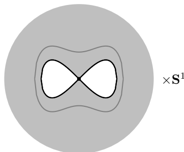
FIGURE 4. Neighbourhood of 8 .
