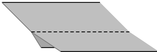
FIGURE 5. Bifurcation complex.
