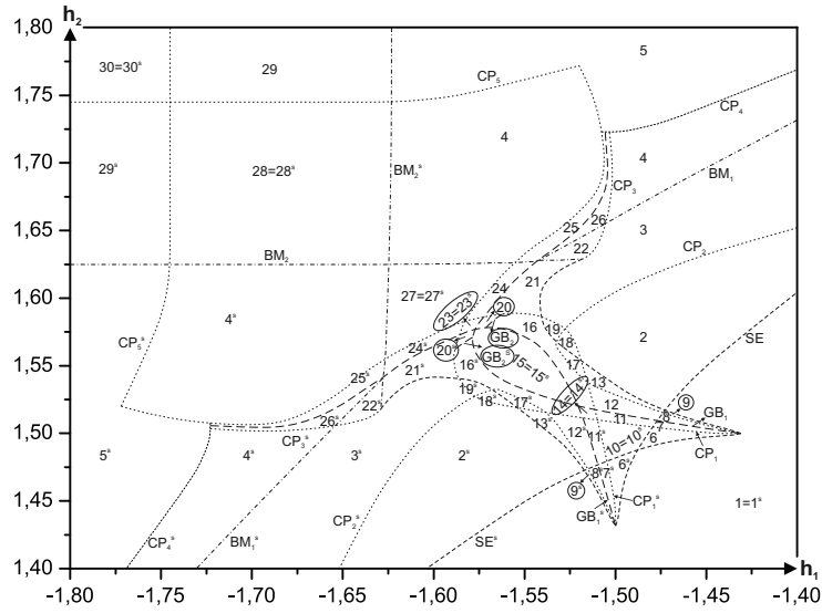
FIGURE 4. Bifurcation diagram for the double lid-driven Z-shaped cavity generated by Çelik [1].
