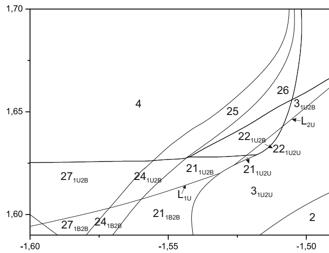
FIGURE 5. Enlarged view of the control space diagram region (Figure 4) where the separation bubble is formed.
