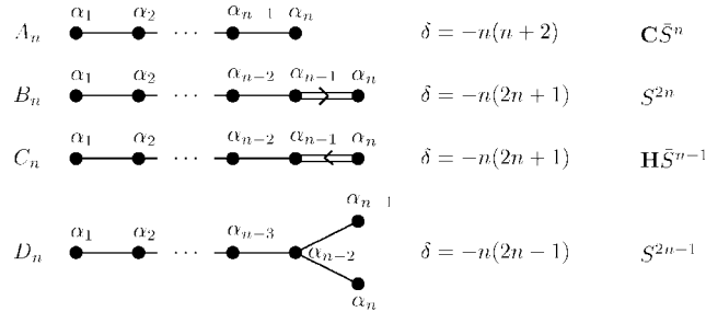
Fig. 1. Dynkin diagrams for classical groups A_n, B_n, C_n, D_n
