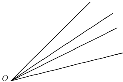
FIGURE 1. A nonnegative cone \mathcal{M}_+ in a linear space \mathcal{A} .
