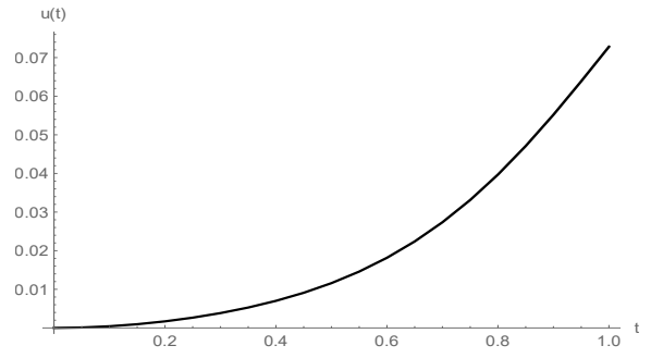
FIGURE 6. Solution curve u(t) for \delta = 3 and \epsilon = 3 .
