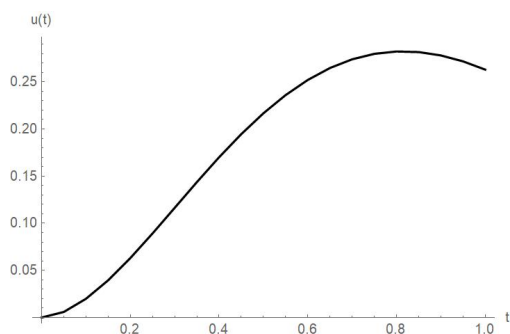
FIGURE 21. Solution curve u(t) for \delta = 2.8 and \epsilon = 2.9 .
