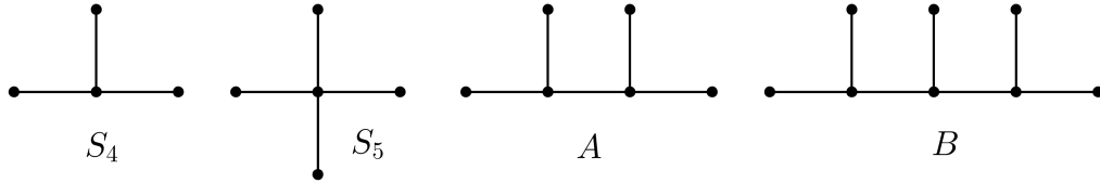
FIGURE 3. Trees S_4 , S_5 , A and B
