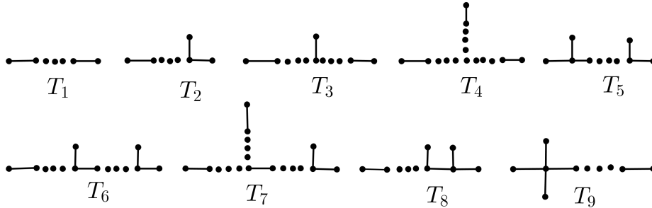
FIGURE 4. Trees in Theorem 3.3
