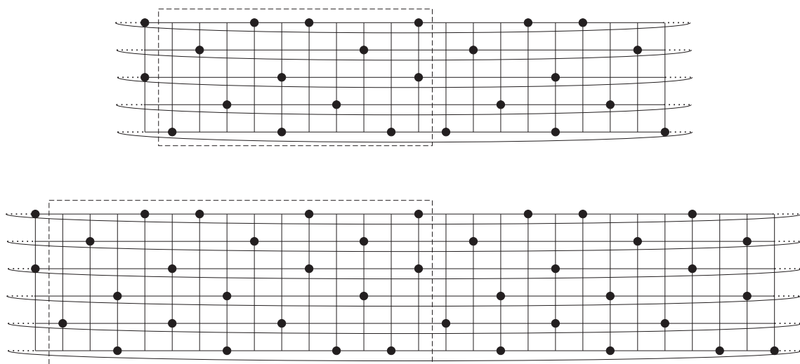
FIGURE 1. Periodical behaviour of \gamma -sets of C_n \square P_k for 5 \leq k \leq 6 .
