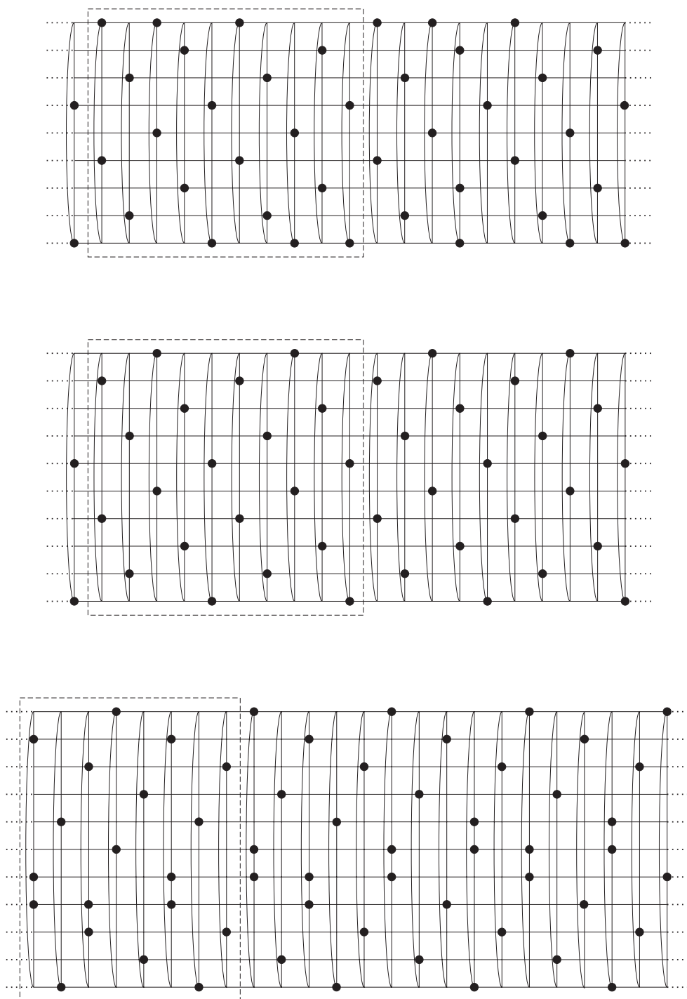
FIGURE 2. Periodical behaviour of \gamma -sets of P_n \square C_k for 9 \leq k \leq 11 .
