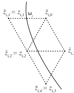
Figure 3: Construction of the polygon \{z_{i,j}\}_{j=1}^{m_i} .
