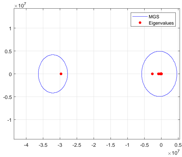
Figure 6: The result of the algorithm iMGSt for the Orr-Sommerfeld matrix of a size n = 1000 .
