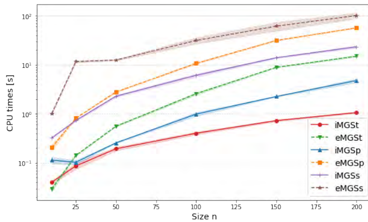
Figure 8: The comparison of CPU times of the algorithms for the Grcar matrices.
