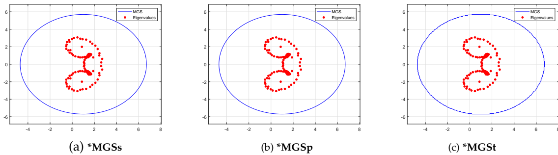
Figure 7: The results of the algorithms for the Grcar matrix of a size n = 100 .
