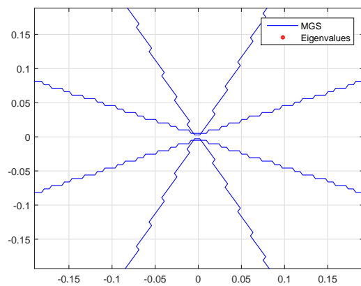
Figure 4: The results of the algorithms for the the cyclic matrix A from Example 5.1: complete plot and plot zoomed around the origin.
