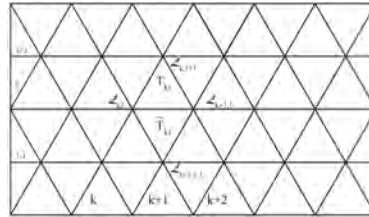
Figure 2: Triangular grid.
