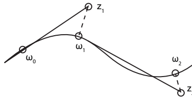
Figure 1: Predictor-corrector step.
