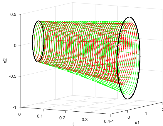
Figure 5. The solution X(t, v^*, u^*) - red, the solution Y(t, v^*, u^*) - green, t \in [0, 0.365] .
