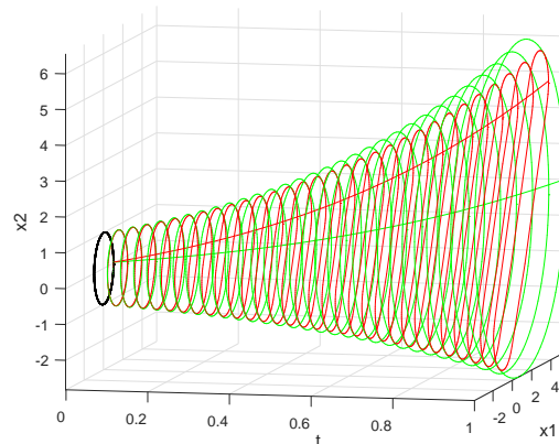
Figure 2. The solution X(t, v, u) - red, the solution Y(t, v, u) - green, t \in [0, 1] .
