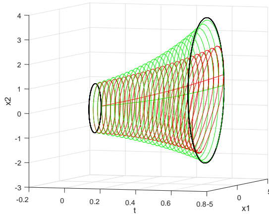
Figure 4. The solution X(t, v^*, u^*) - red, the solution Y(t, v^*, u^*) - green, t \in [0, 0.665] .
