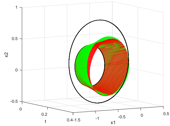
Figure 10. X(t, v^*, u^*) - red, Y(t, v^*, u^*) - green, t \in [0, 0.248]
