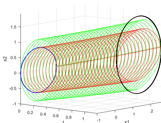
Figure 11. X_0 - blue, X_K - black, X(t, v^*, u^*) - red, Y(t, v^*, u^*) - green, t \in [0, 1.19]
