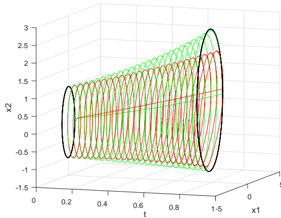
Figure 8. The solution X(t, v^*, u^*) - red, the solution Y(t, v^*, u^*) - green, t \in [0, 0.83]
