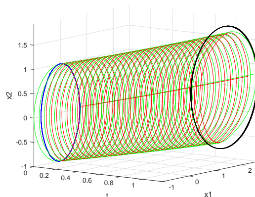
Figure 12. X_0 - blue, X_K - black, X(t, v^*, u^*) - red, Y(t, v^*, u^*) - green, t \in [0, 1.19]
