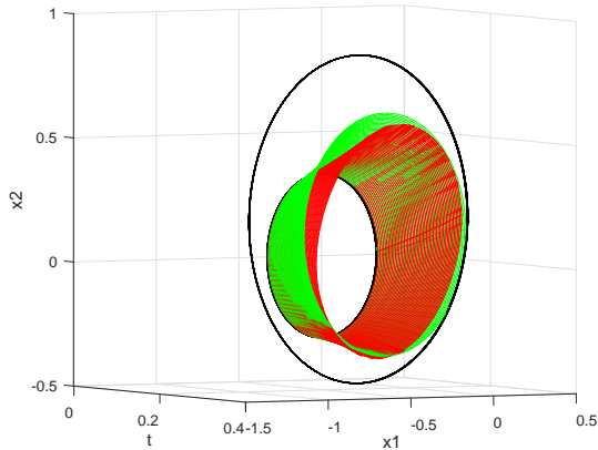
Figure 9. X(t, v^*, u^*) - red, Y(t, v^*, u^*) - green, t \in [0, 0.275]
