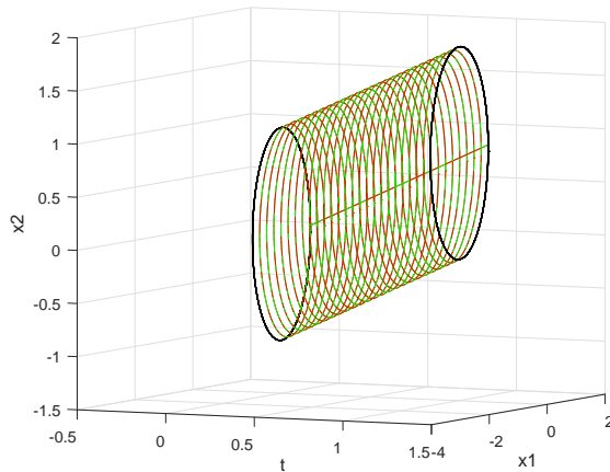
Figure 3. The solution X(t, v^*, u^*) , t \in [0, 1.2] .
