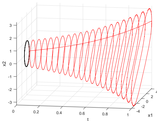
Figure 1. The solution X_1(t) , t \in [0, 1] .
