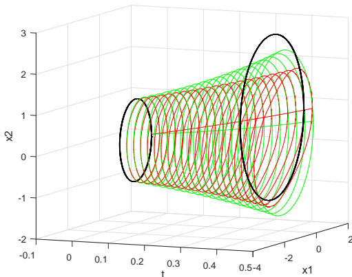
Figure 6. X(t, 1, u^*) - red, Y(t, 1, u^*) - green, t \in [0, 0.43] .
