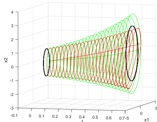
Figure 7. X(t, 1, u^*) - red, Y(t, 1, u^*) - green, t \in [0, 0.665] .
