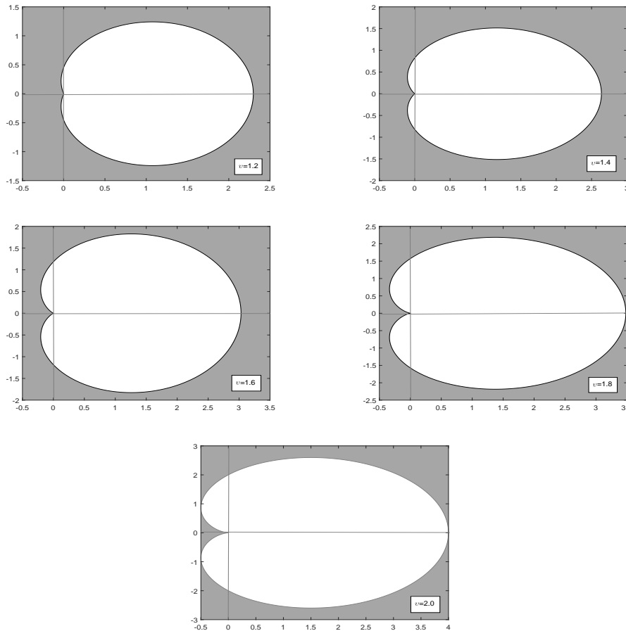
Figure 1: Stability regions (the grey areas) for the proposed method in Eq.(3.13) for v = 1.2, 1.4, 1.6, 1.8, 2 .
