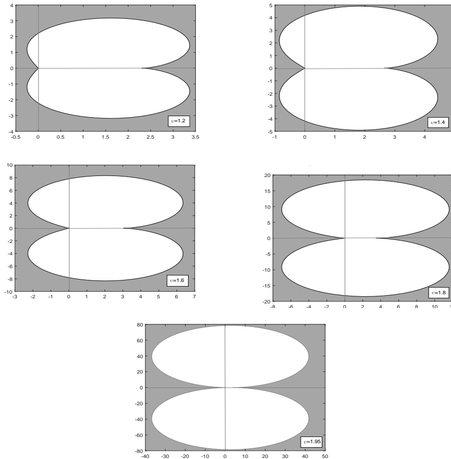
Figure 2: Stability regions (the grey areas) for the proposed method in Eq.(3.14) for v = 1.2, 1.4, 1.6, 1.8, 1.95 .
