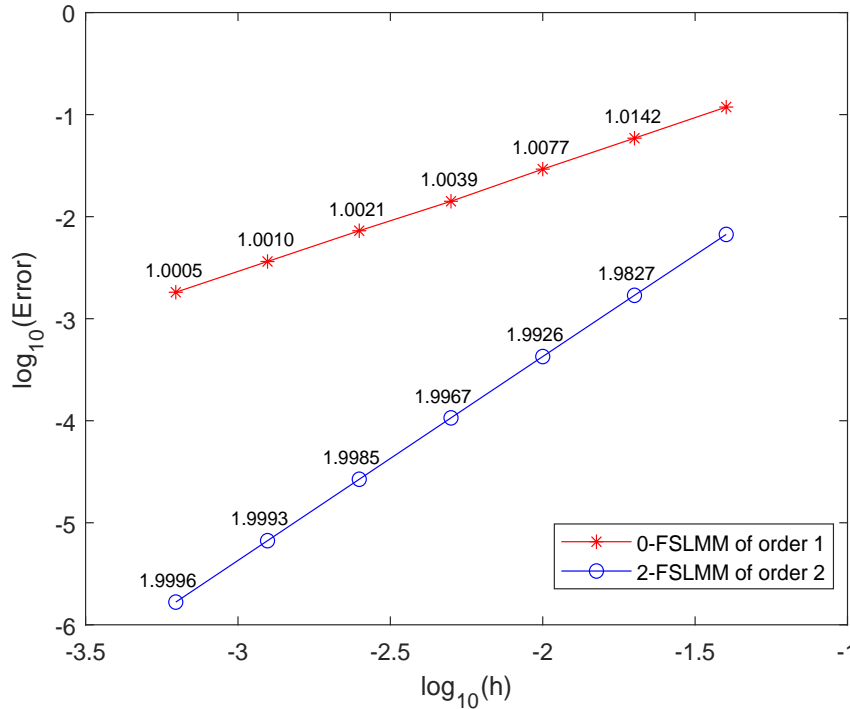
Figure 5: Errors and order of convergence for Example 2 at t = 1 for v = 1.6 and h = \frac{1}{25}, \frac{1}{50}, \dots, \frac{1}{1600} .
