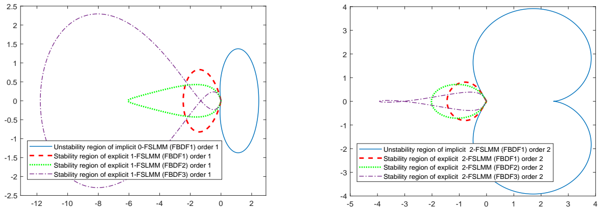
Figure 3: Comparison the stability regions of implicit proposed methods (outside of the closed regions) and explicit methods [15] (inside of the closed regions) for \nu = 1.3 .
