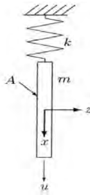
Figure 6: The immersed plate into a Newtonian fluid .
