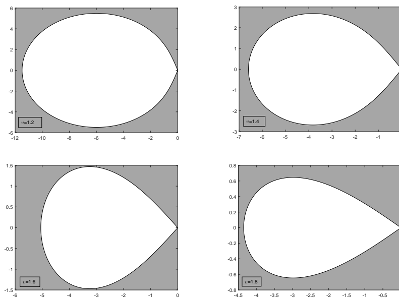
Figure 4: Stability regions (the grey areas) for the proposed method in Eq.(3.23) for \nu = 1.2, 1.4, 1.6, 1.8 .
