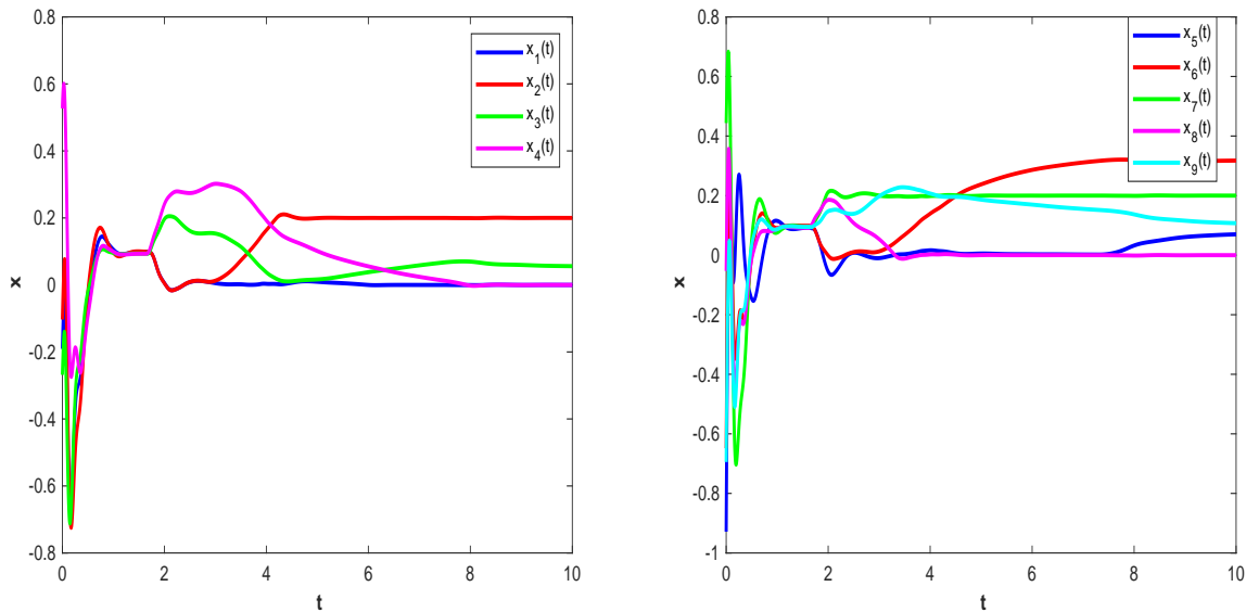
Figure 1: Transient behaviors of x_1(t), \dots, x_9(t) with r_0 = 0.05 for the problem (9).
