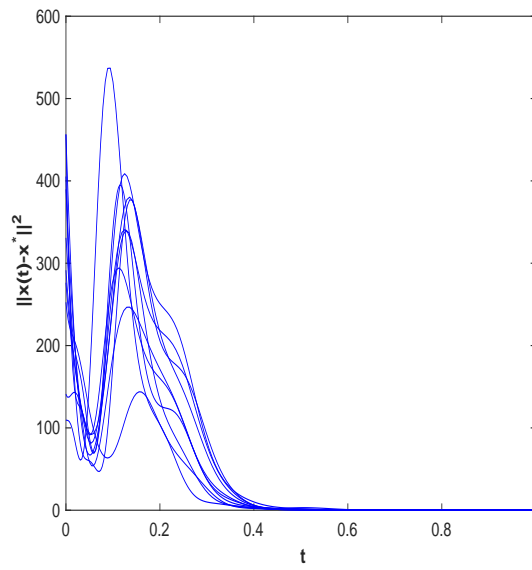
Figure 5: The convergence behavior of \|x(t) - x^*\|^2 with \eta = 15 , 10 different initial points and r_0 = 0.05 for the problem (9).
