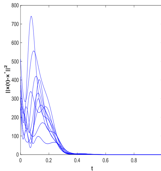
Figure 6: The convergence behavior of \|x(t) - x^*\|^2 with \eta = 15 , 10 different initial points and r_0 = 0.05 for the problem (10).
