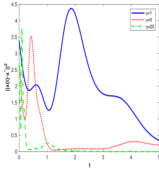
Figure 4: Convergence behavior of \|x(t) - x^*\|^2 with different values of \eta and r_0 = 0.05 for the problem (10).
