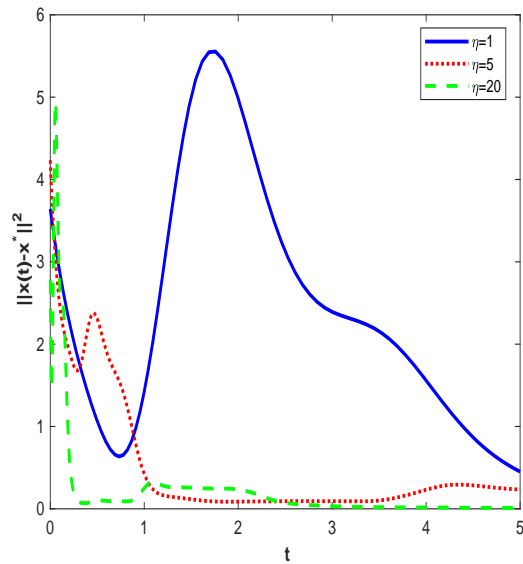
Figure 3: Convergence behavior of \|x(t) - x^*\|^2 with different values of \eta and r_0 = 0.05 for the problem (9).
