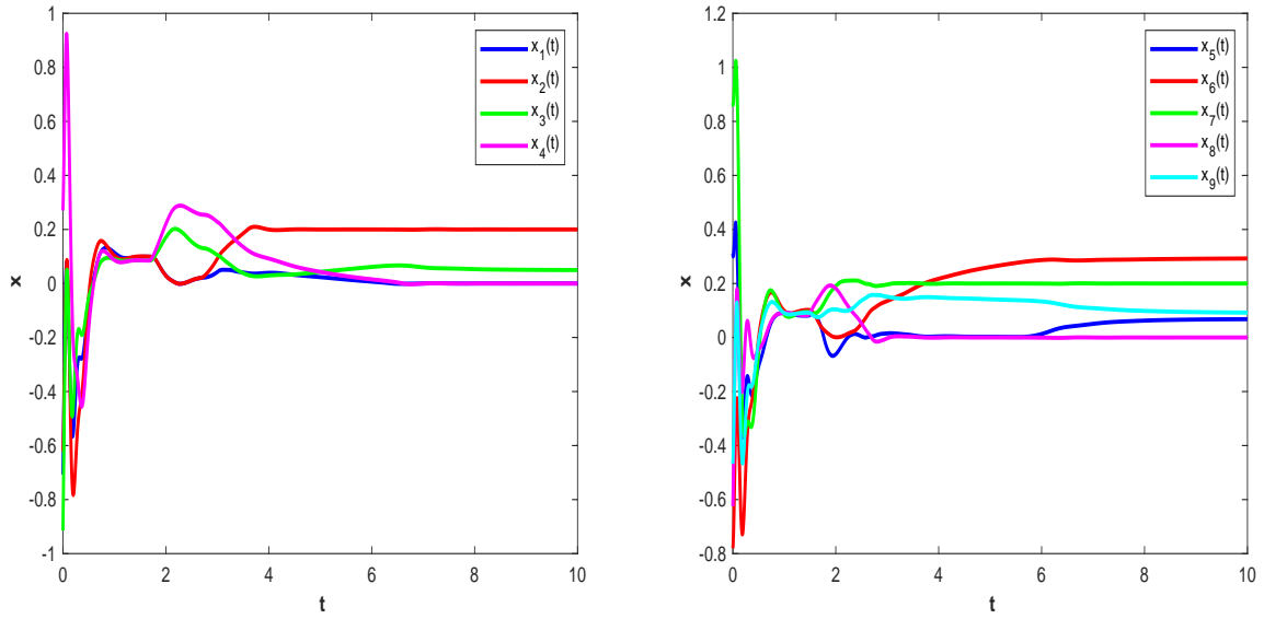
Figure 2: Transient behaviors of x_1(t), \dots, x_9(t) with r_0 = 0.05 for the problem (10).
