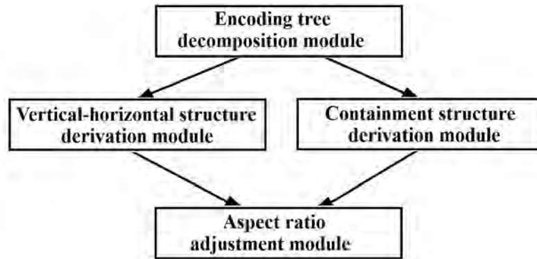
Fig. 5. Structure of the intelligent derivation mechanism.
