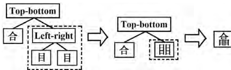
Fig. 6. Intelligent derivation process of w_6 .
