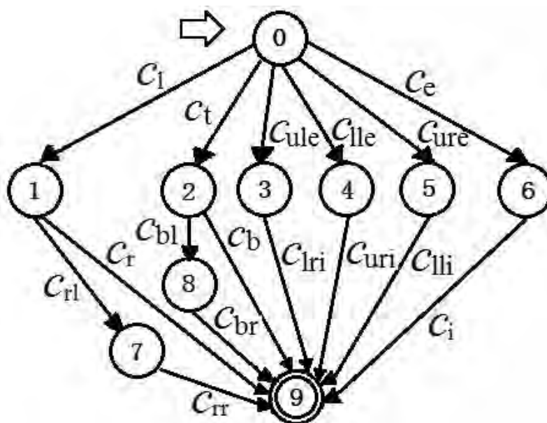
Fig. 2. State graph to generate square Hmong characters.
