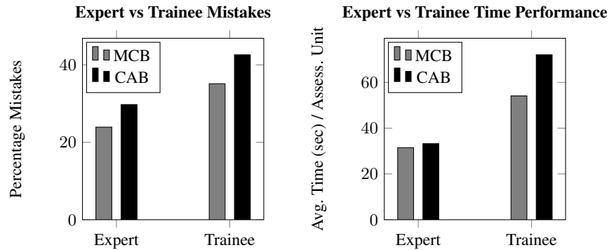
Fig. 10. Manual vs Content-Agnostic Results
