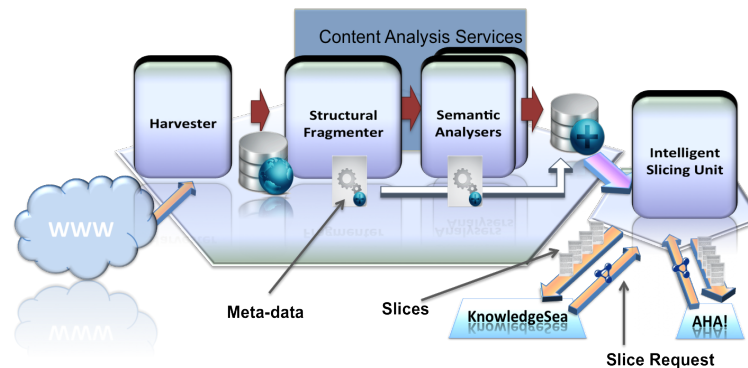
Fig. 1. Slicer Anatomy
