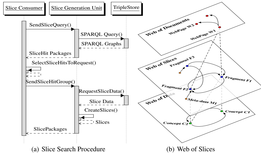
Fig. 3. Slice Generation
