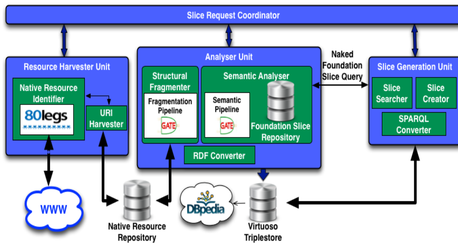
Fig. 2. Slicepedia Implementation
