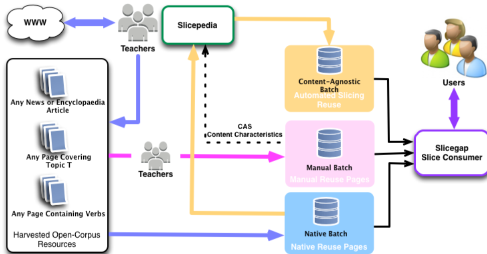
Fig. 5. SliceGap Content Batch Creation
