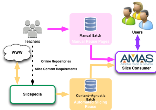
Fig. 6. AMAS Content Batch Creation
